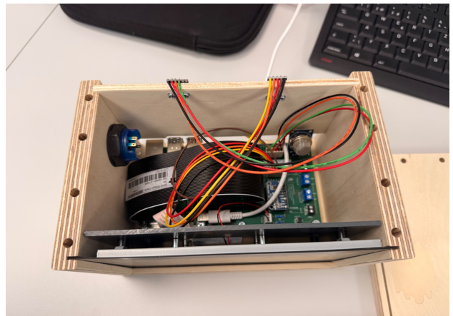
Top view — internal wiring and components
