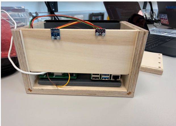
Rear view — sensors and Raspberry Pi
